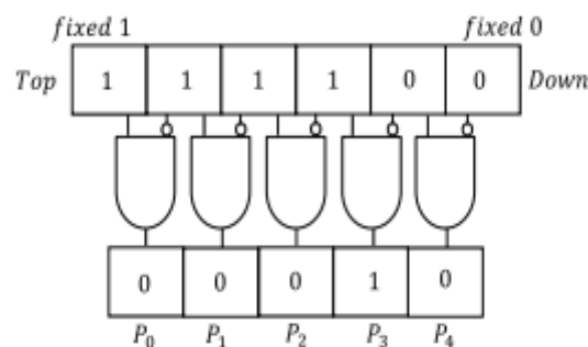
Fig. 7 One-hot code generation circuit.
