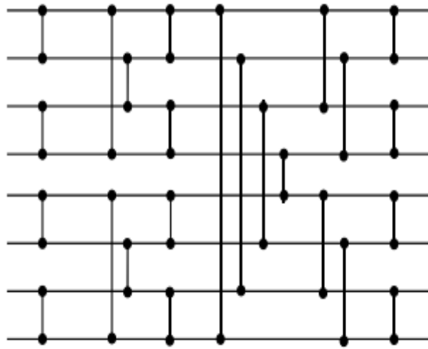
Fig10 Eight-way sorting network.
