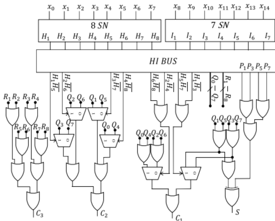
Fig.9 Overall (15,4) counter circuit
